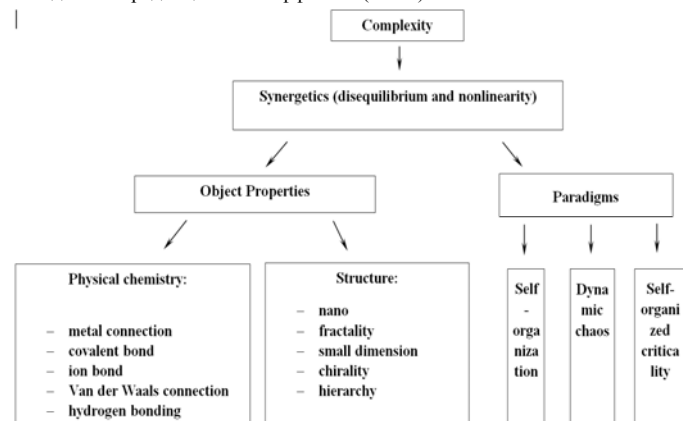
Fig.1. Scheme of the extended concept of "Complexity" as applied to radiation effects in complex media.
