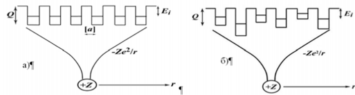
Fig.2. Scheme of the Coulomb effect of the Auger charge on the electronic potential relief of a strictly periodic (a) and in an aperiodic Anderson chain (b).
